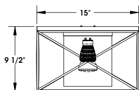
TIC TACK FIXTURE # 663.01 15" square x 9.5" drop GU24 socket for 23w CFL or LED bulb shown in Brushed Nickel finish, with seamless opal acrylic at side and bottom
