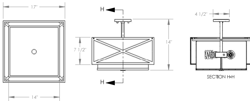
CUSTOM FIXTURE for Xavier Yager, Lightology, Chicago. Nested lampshades with 4 standard base sockets. Remove bottom button to access bulbs.
