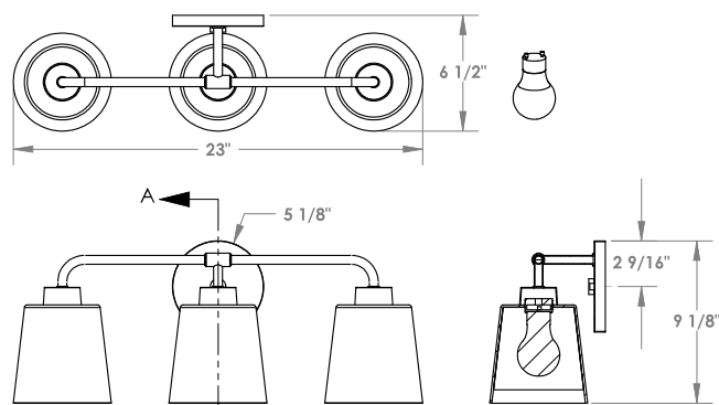
VANITY 3-LIGHT SCONCE # C1485-POLN-DKOX in Polished Nickel finish with black accents 23" wide x 9.1" tall x 6.5" extension white glass shades are clear at bottom 10w. GU24 sockets for LED bulbs
