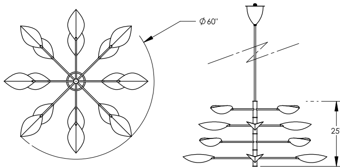
Mineola Chandelier # C1919 60" diameter x 25" tall (main body), overall drop TBD 16 x E12 (candelabra) sockets for 6w LED bulbs by others Dark Oxide (black) painted finish & Medium Antique Brass patina UL/ETL certification
