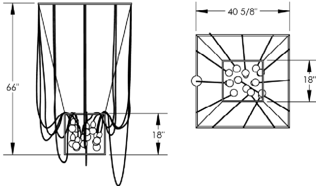
Firefly Trap, Swag Chandelier # C2170 40.6" x 40.6" x 66" overall drop 12 x E26 sockets for G40 LED bulbs (by others) Dark Oxide (black) finish and custom color on the sockets UL/ETL certification
